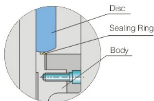
Elastic Ring Hard Seal Structure (Fig.c)
