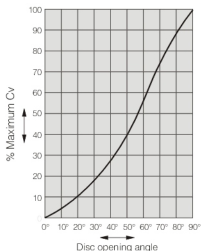
Typical Characteristic Curve of High Performance Butterfly Valve
