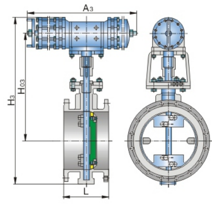
Pneumatic Flanged Butterfly Valve
