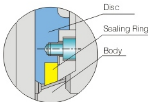
Soft Sealing Structure (Fig.a)
