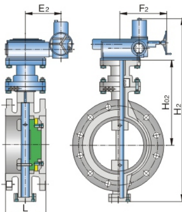
Electric Flanged Butterfly Valve
