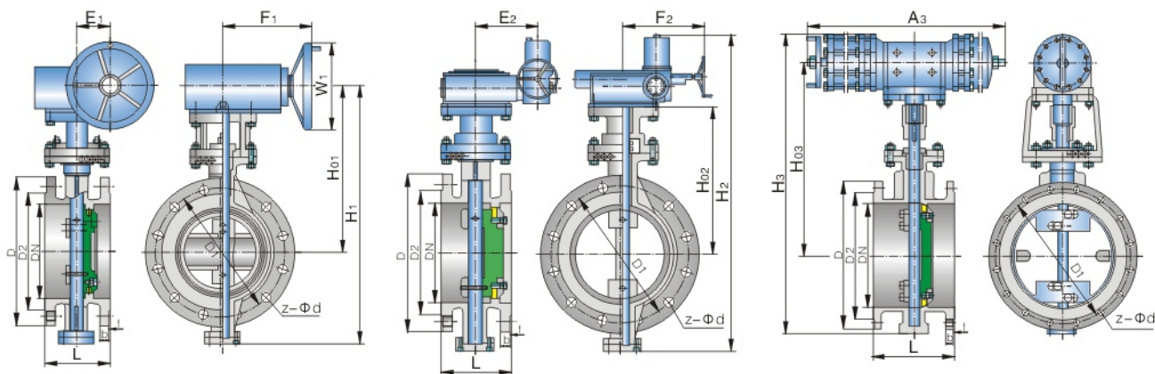
Worm Gear Flanged Butterfly Valve
