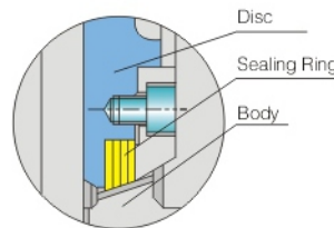
Multilayer Hard Seal Structure (Fig.b)
