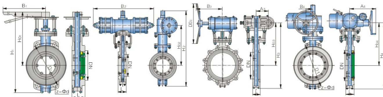
Manual Wafer Butterfly Valve
