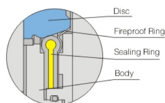
Soft Seal Fireproof Structure (Fig.d)
