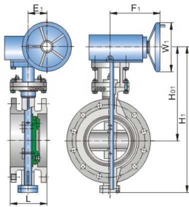
Worm Gear Flanged Butterfly Valve
