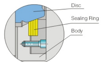
Multilayer Hard Seal Structure (Fig.b)
