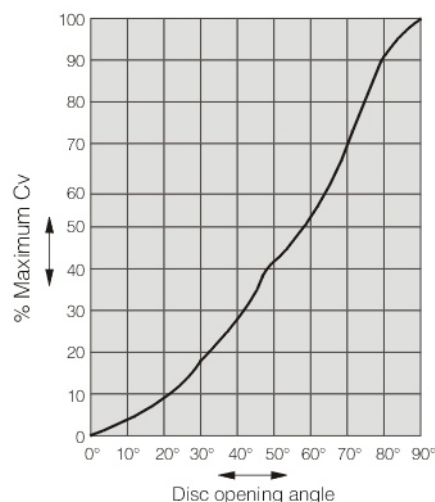
Typical Characteristic Curve of Double Eccentric Hard Butterfly Valve
