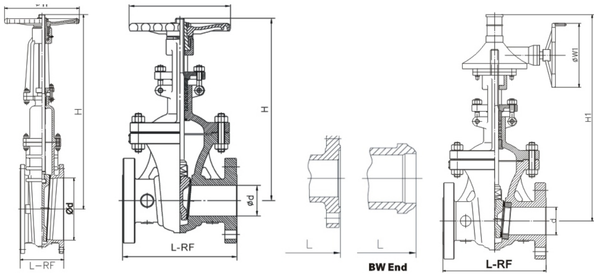
PN10(DIN 3202-F4)
